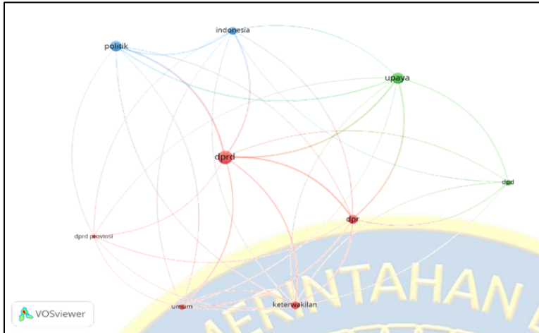
Gambar 1. Vosviewer Penelitian
